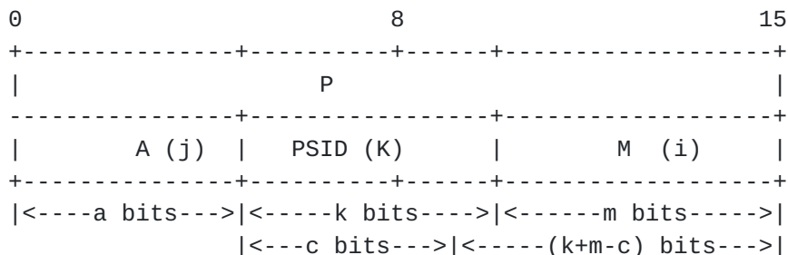
Figure 2: Bit representation
