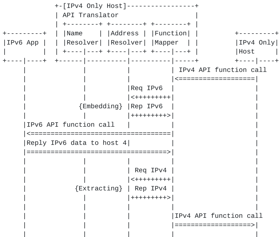
Figure 8: Behavior of receiving data from IPv4 host
