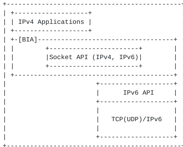
Figure 1: the architecture of IPv6 only host In which BIA is installed.
