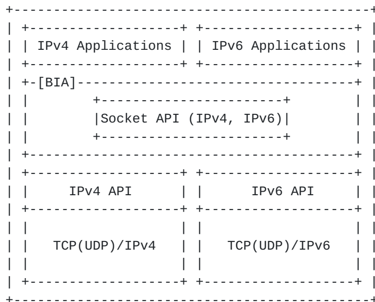
Figure 3: the architecture of dual stack host In which BIA is installed.
