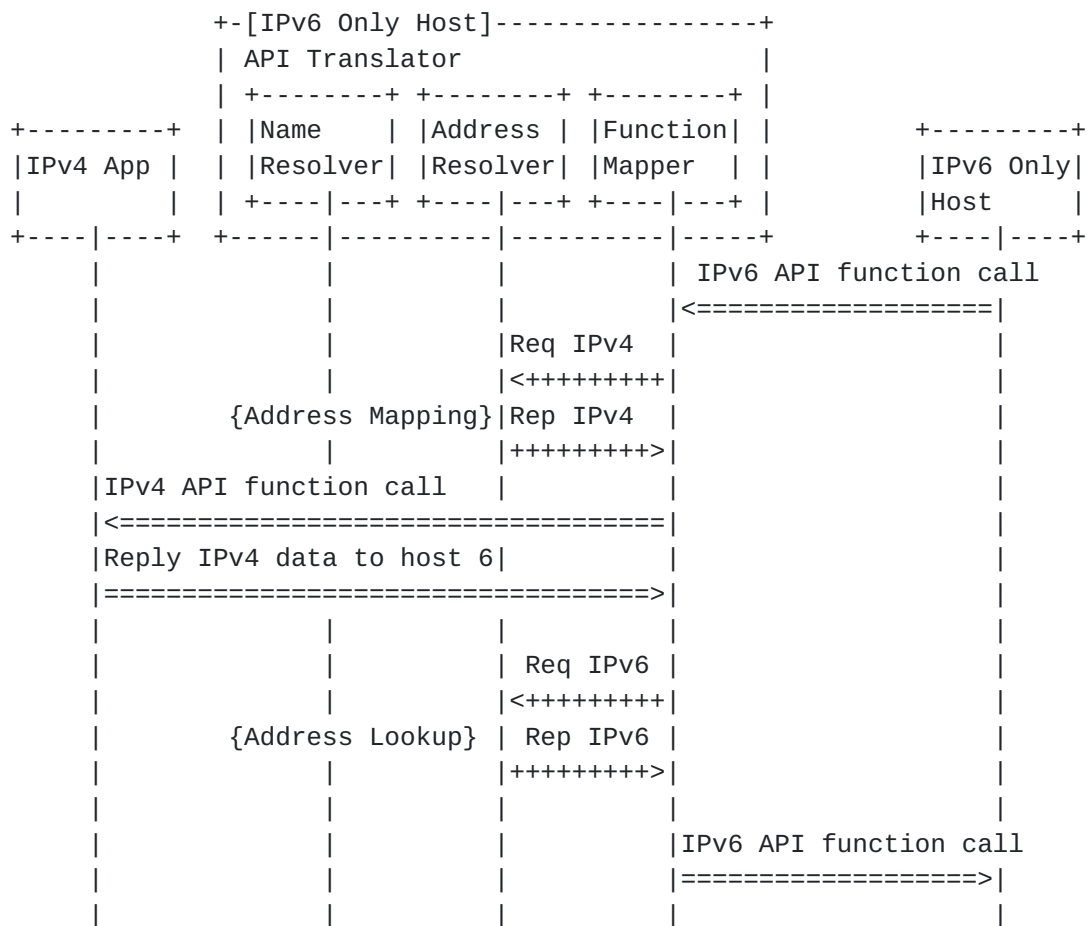
Figure 6: Behavior of receiving data from IPv6 host
