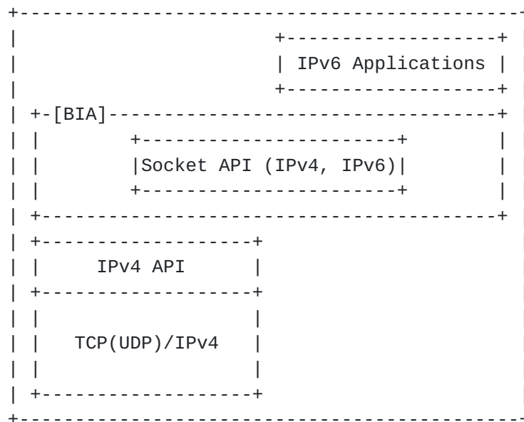
Figure 2: the architecture of IPv4 only host In which BIA is installed.
