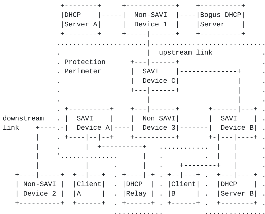
Figure 1: SAVI-DHCP Scenario
