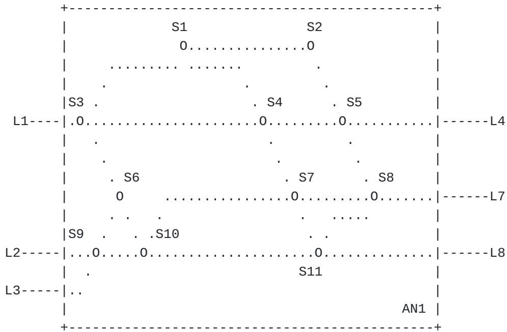
Figure 3: Type 2 topology
