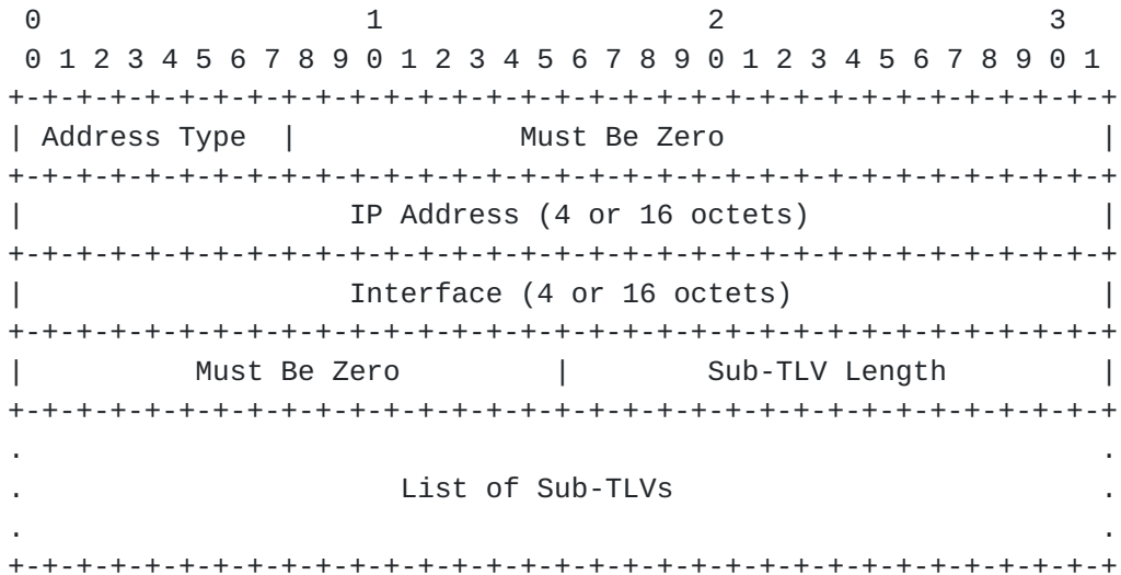
Figure 5: Detailed Interface and Label Stack TLV
