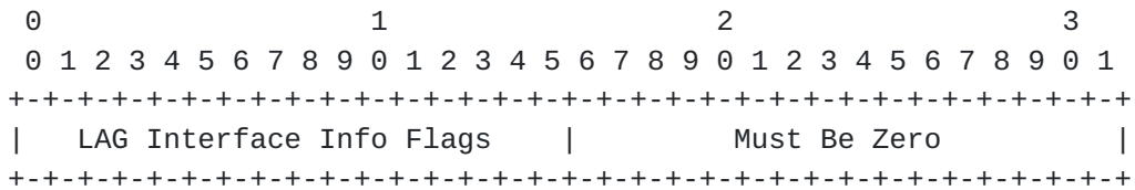
Figure 3: LAG Interface Info TLV
