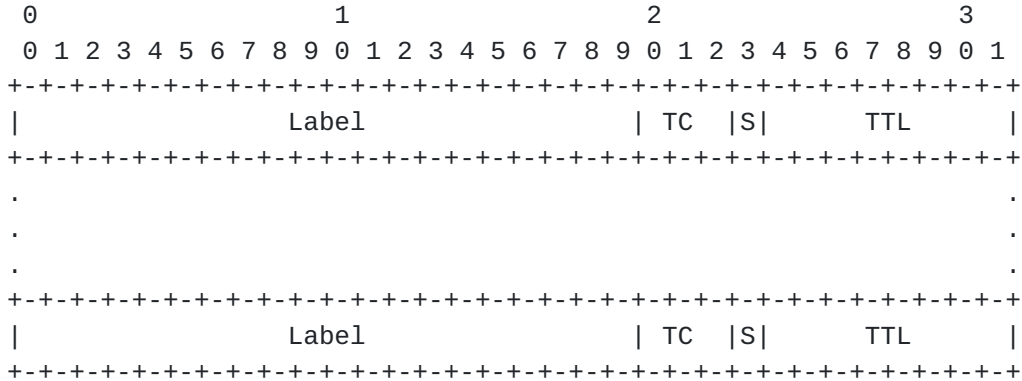
Figure 6: Incoming Label Stack Sub-TLV
