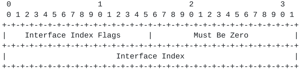
Figure 7: Incoming Interface Index Sub-TLV
