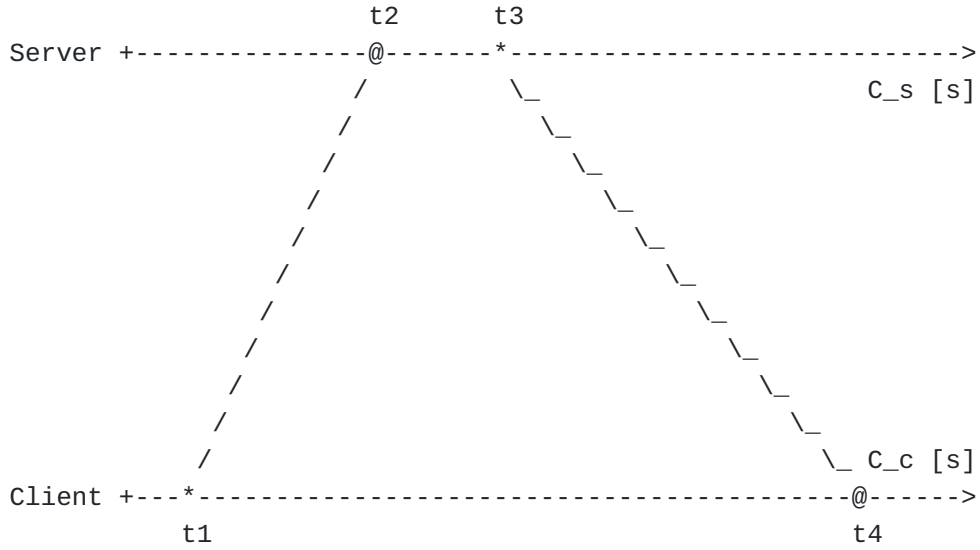
Figure 2: Time line of packets.--
