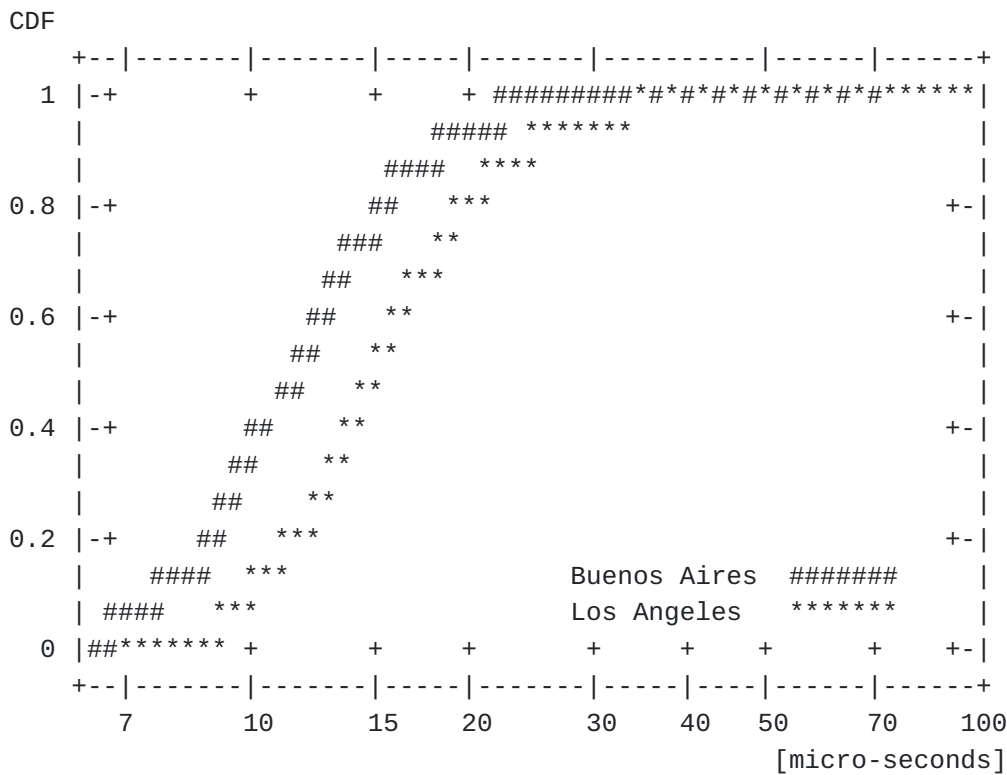
Figure 9: Cumulative distribution function of the MTIE (60s).--
