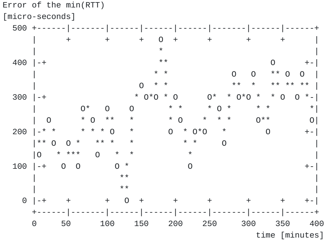
Figure 3: Min RTT error, estimated every 10 minutes along 7 hours.--
