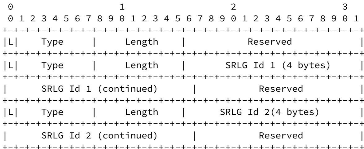
Figure 1: Example of EIRS with SRLG subobjects
