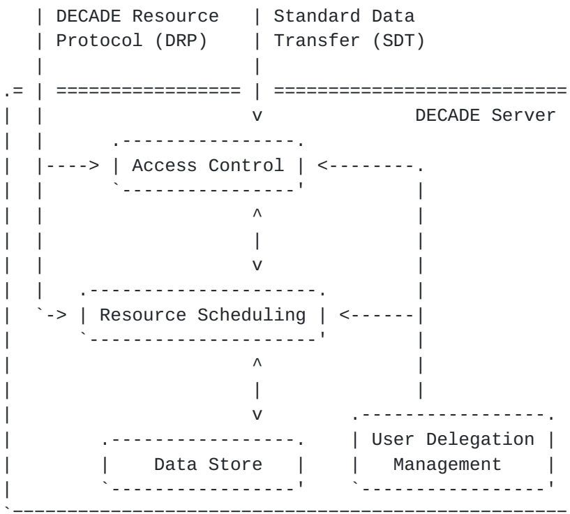
Figure 4: DECADE Server Components
