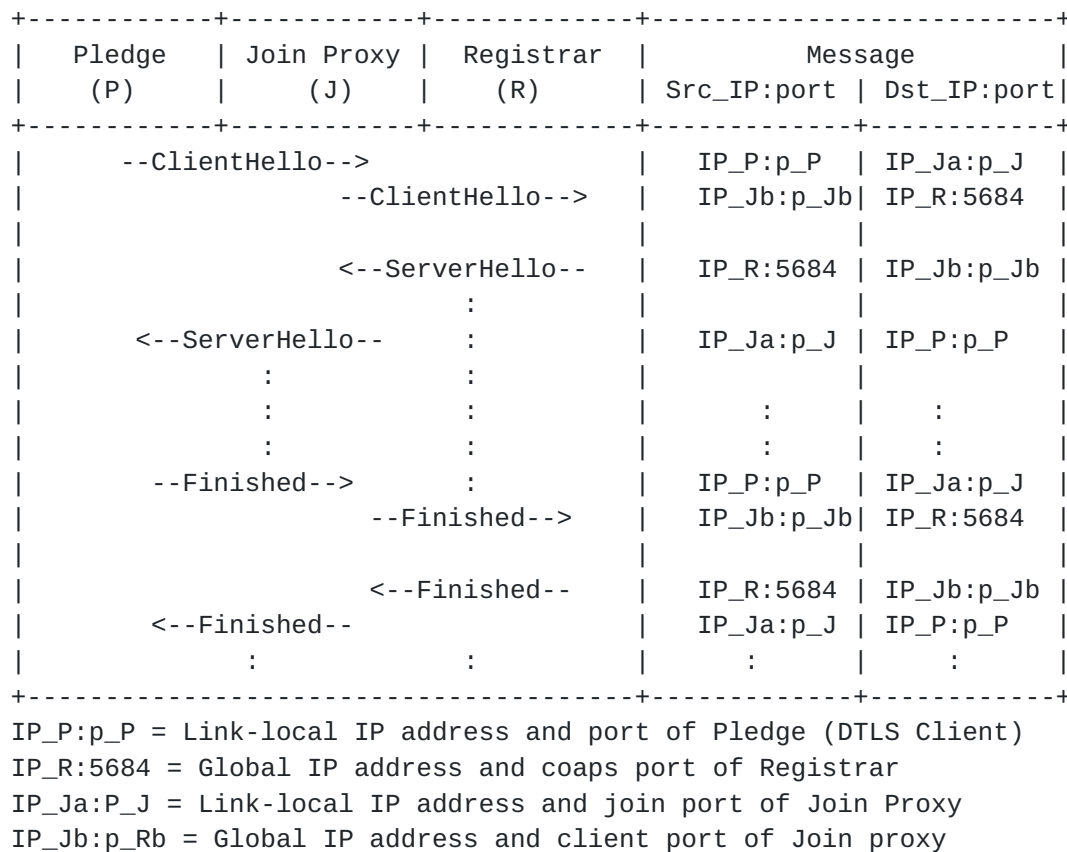
Figure 2: constrained statefull joining message flow with Registrar address known to Join Proxy.
