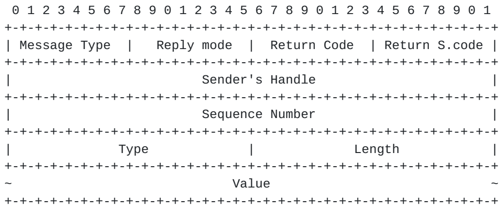
Figure 1: COAM Packet Header
