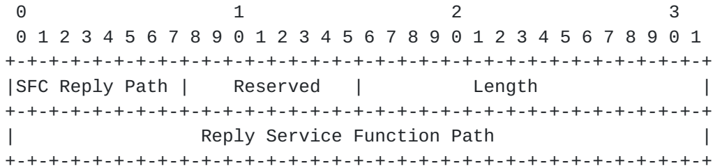
Figure 1: SFC Reply TLV Format
