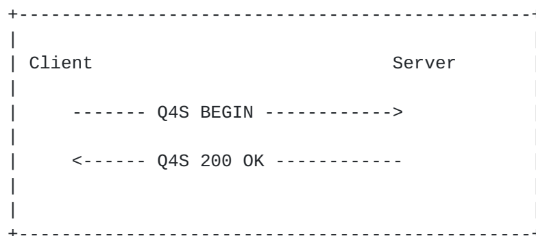
Figure 7 Handshake phase.
