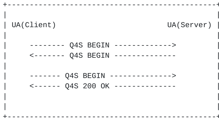
Figure 15 P2P roles.
