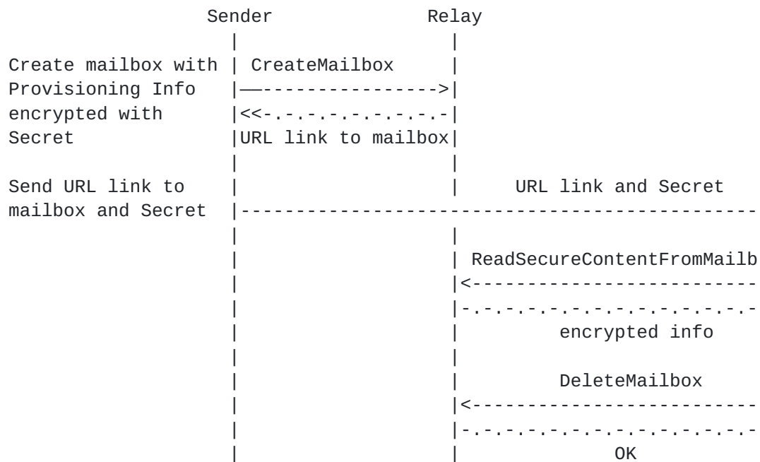
Figure 1: Sample stateless workflow
