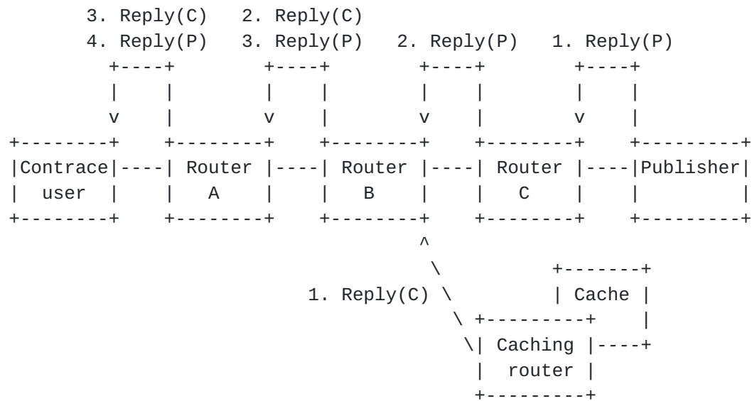
Figure 2: Reply messages forwarded by publisher and routers. Each router forwards the Reply message, and finally the Contrace user receives two Reply messages: one from the publisher and the other from the caching router.
