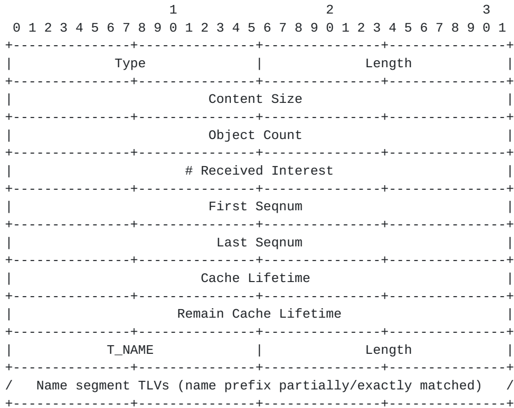
Figure 15: Reply sub-block TLV for T_TRACE_CONTENT and T_TRACE_CONTENT_OWNER (packet payload)
