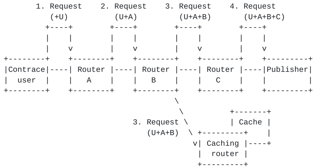
Figure 1: Request messages forwarded by consumer and routers. Contrace user and routers (i.e., Router A,B,C) insert their own Report blocks into the Request message and forward the message toward the content forwarder (i.e., caching router and publisher)
