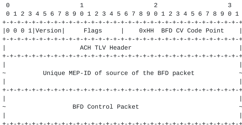
Figure 3: MPLS CV Message
