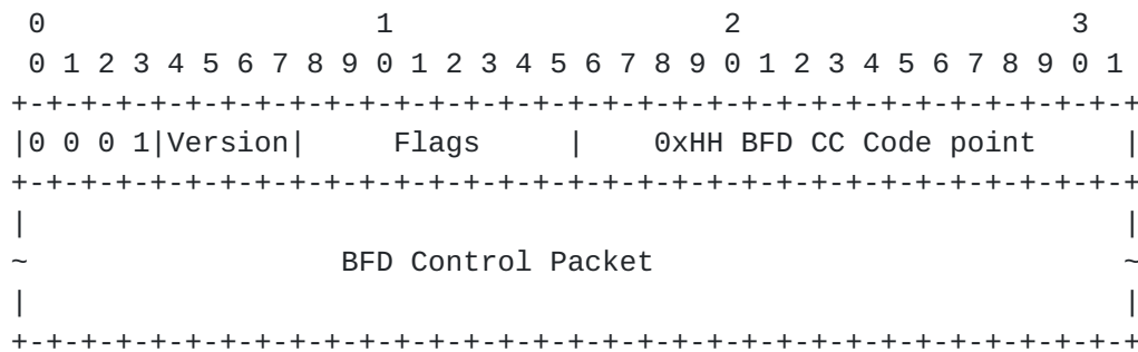
Figure 2: MPLS CC Message
