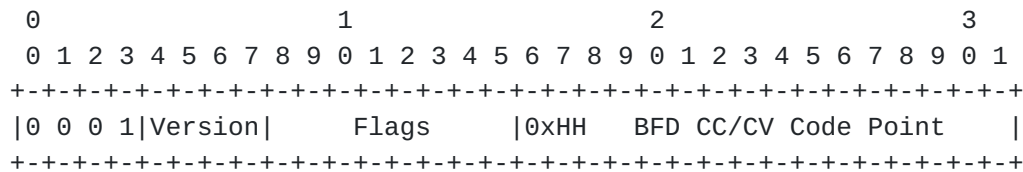
Figure 1: ACH Indication of MPLS-TP Connection Verification
