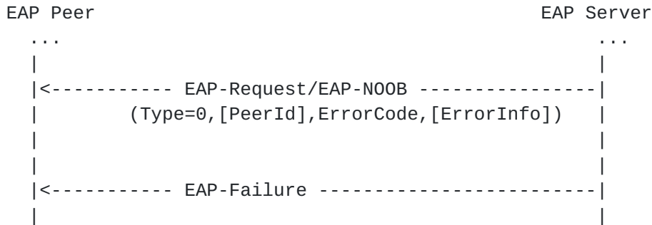
Figure 8: Error notification from server to peer
