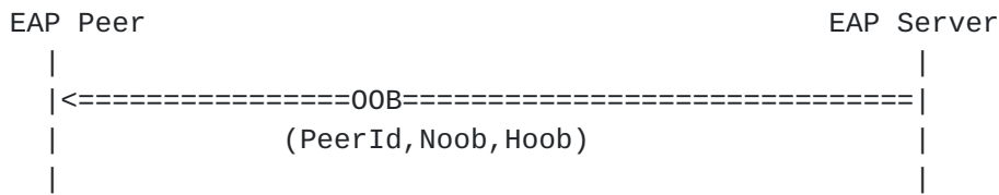
Figure 5: OOB Step, from EAP server to peer
