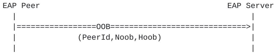
Figure 4: OOB Step, from peer to EAP server
