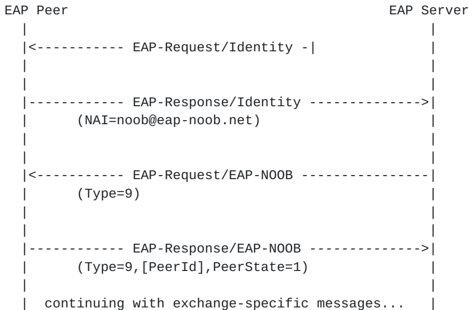
Figure 2: Common handshake in all EAP-NOOB exchanges
