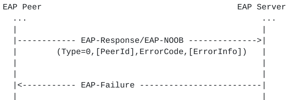
Figure 10: Error notification from peer to server
