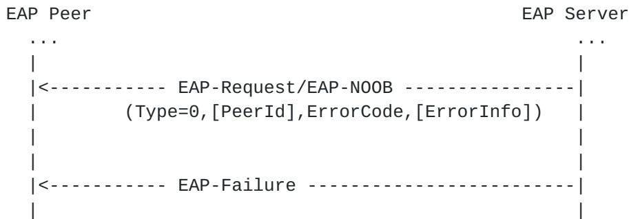
Figure 9: Error notification from server to peer
