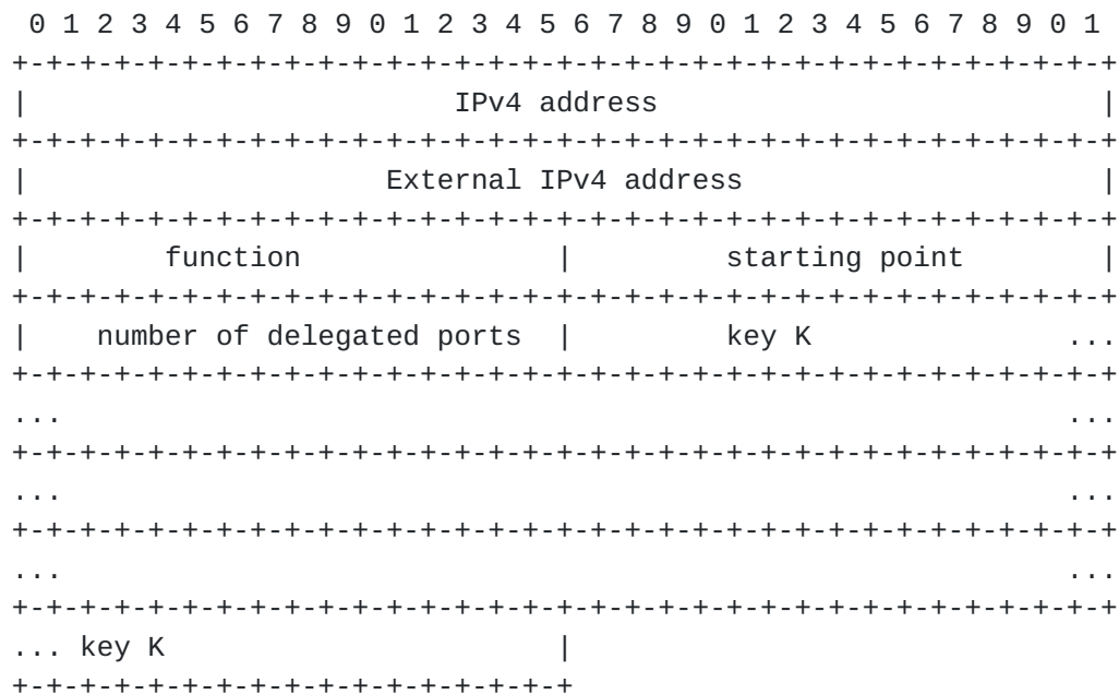
Figure 5: External IP Address with random port sub-option
