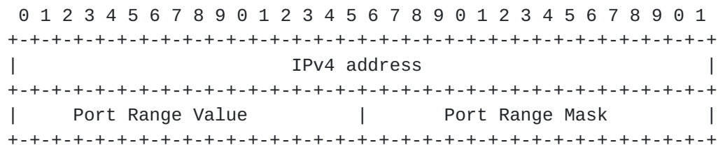
Figure 3: Port Range sub-option
