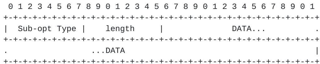
Figure 2: Port Restricted IP Address Sub-option layout
