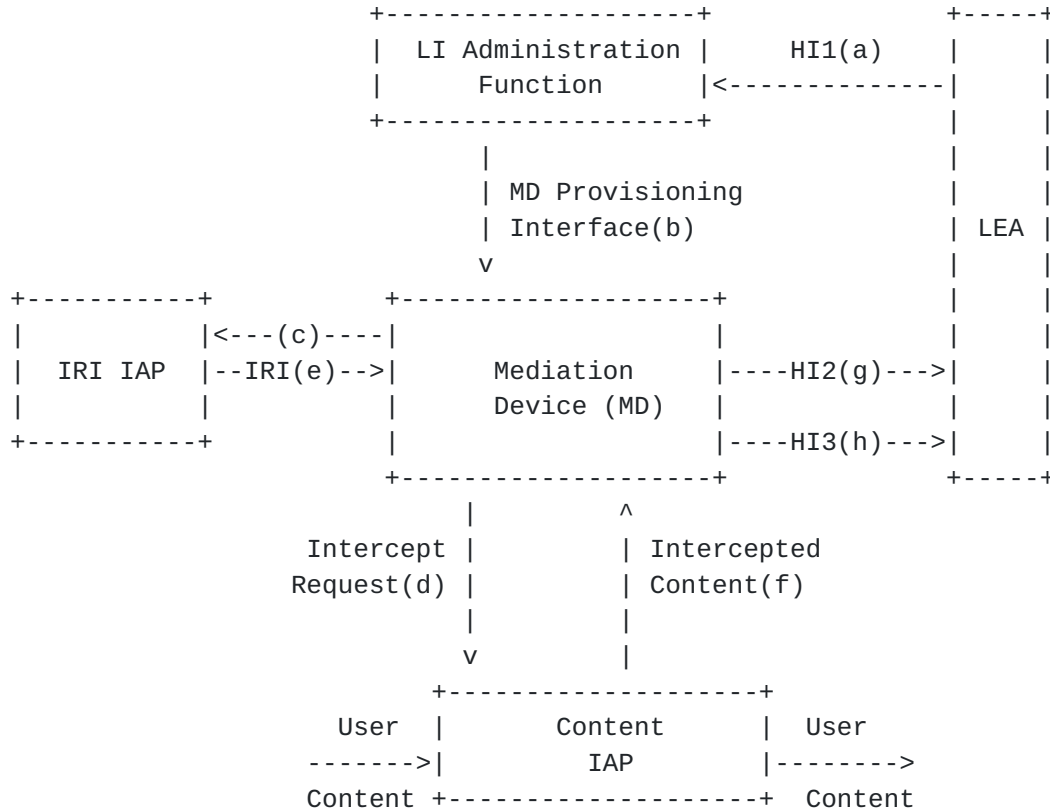
Figure 1: Intercept Architecture
