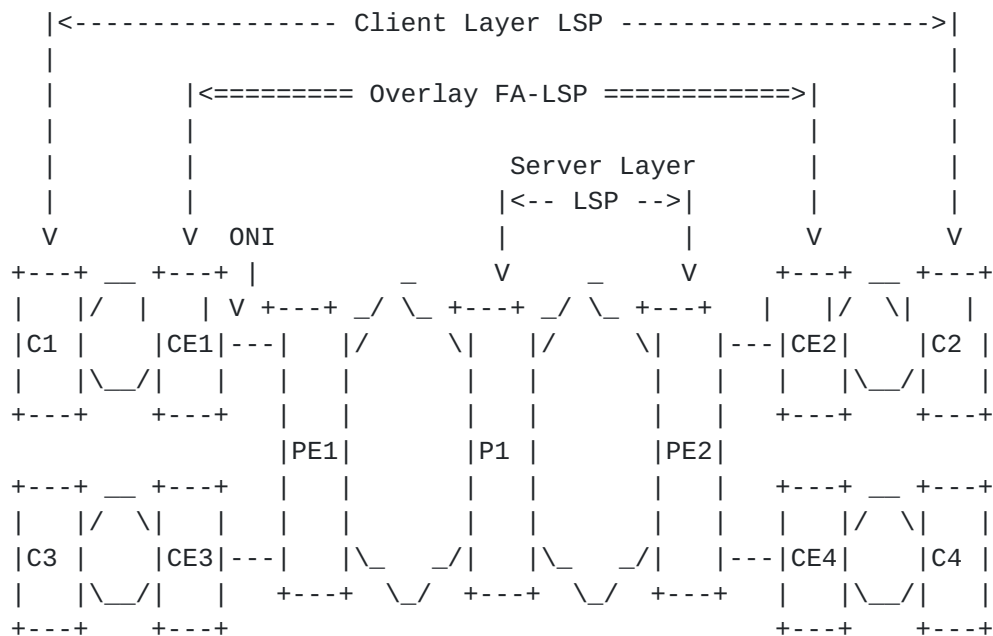
Figure. 2 In Figure 2, the Packet switching continues from customer to provider network and transitions to OTN/DWDM at P1. This kind of configuration is possible in multi-party client and server network, where the provider operates multi-layer network and provide services to its customers.
