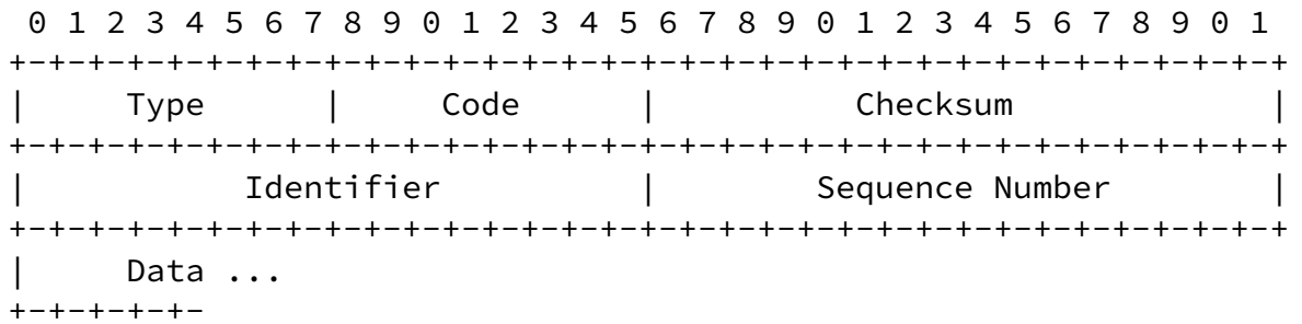
Figure 4: ICMPv6 Echo Request message format
