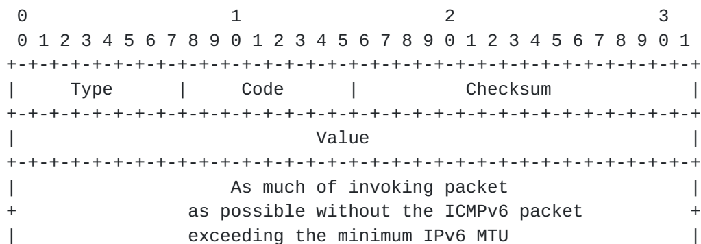
Figure 3: ICMPv6 Error Message format
