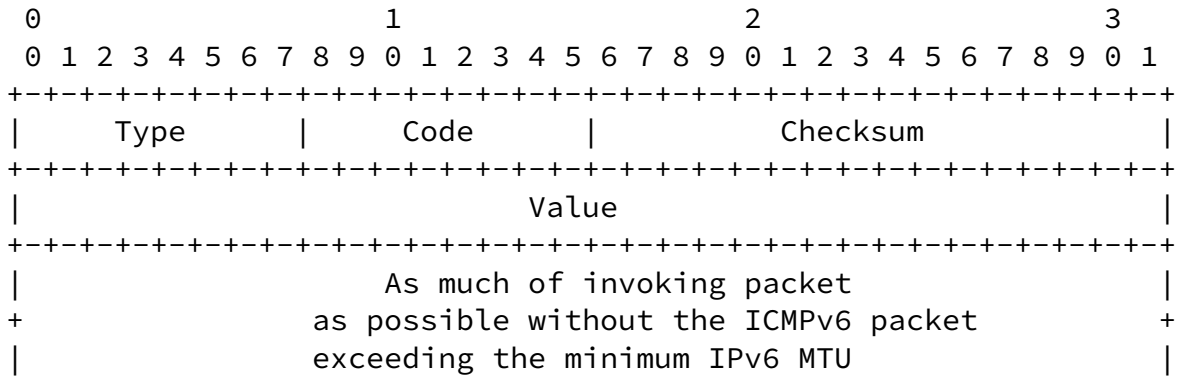
Figure 3: ICMPv6 Error Message format
