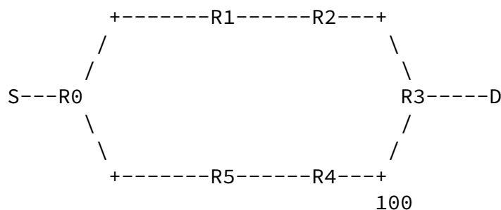
Figure 1 Illustrative scenario, failure of link R2-R3
