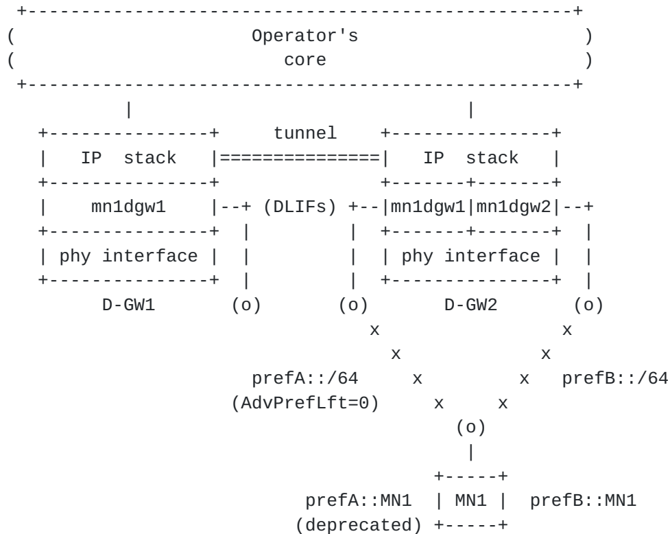
Figure 2: DLIF: exposing multiple routers (one per active anchoring D-GW)
