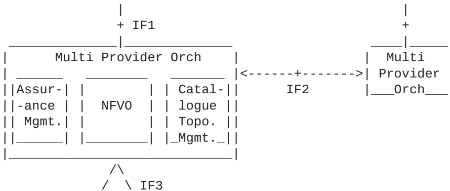
Figure 12: Detailed MPO reference architecture
