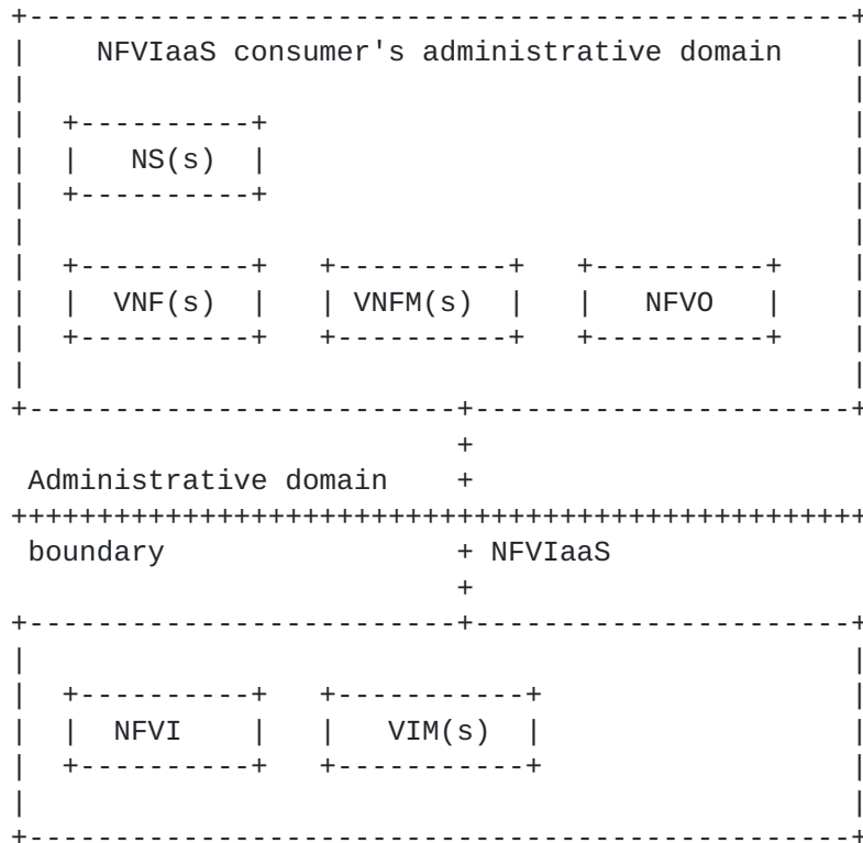
Figure 5: NFVI use case
