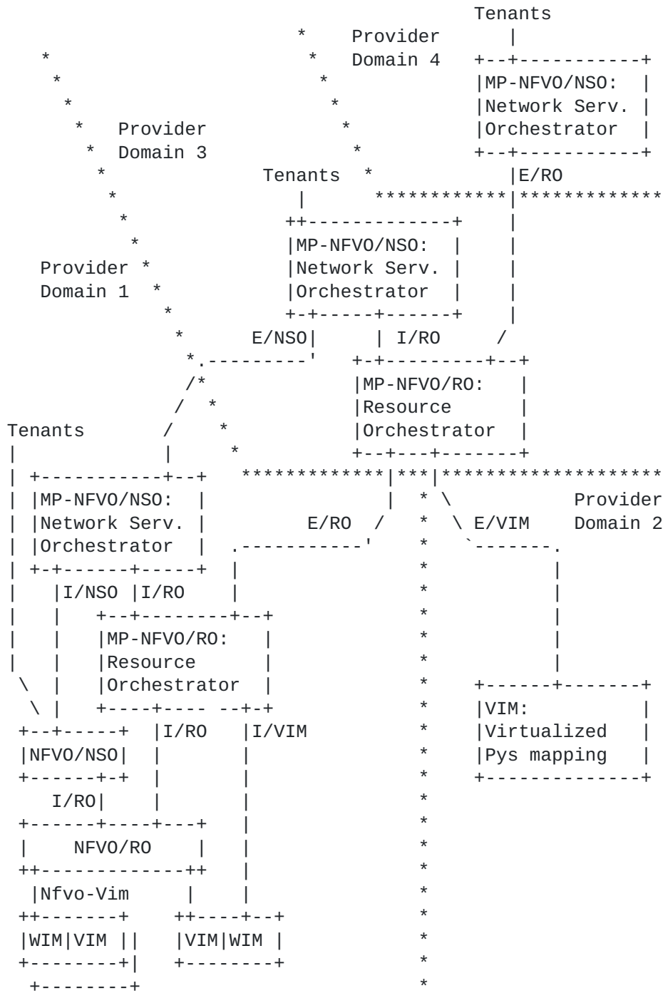
Figure 10: NSO-RO Split: possible multi-provider APIs - an illustration
