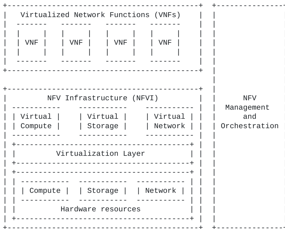
Figure 1: ETSI NFV framework
