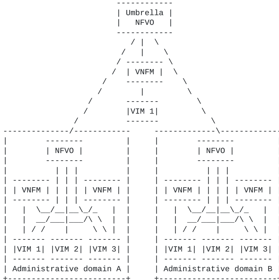
Figure 4: Network services provided using multiple administrative domains (from ETSI GS NFV-IFA 009 V1.1.1)
