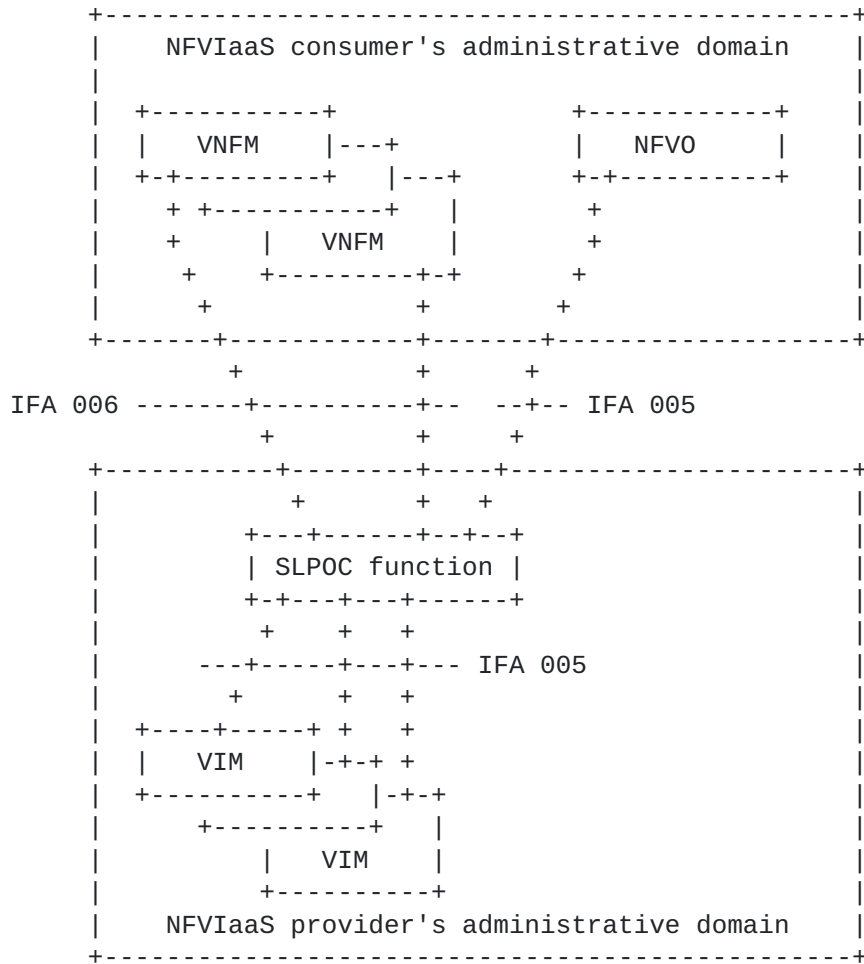
Figure 7: NFVIaaS architecture: SLPOC option
