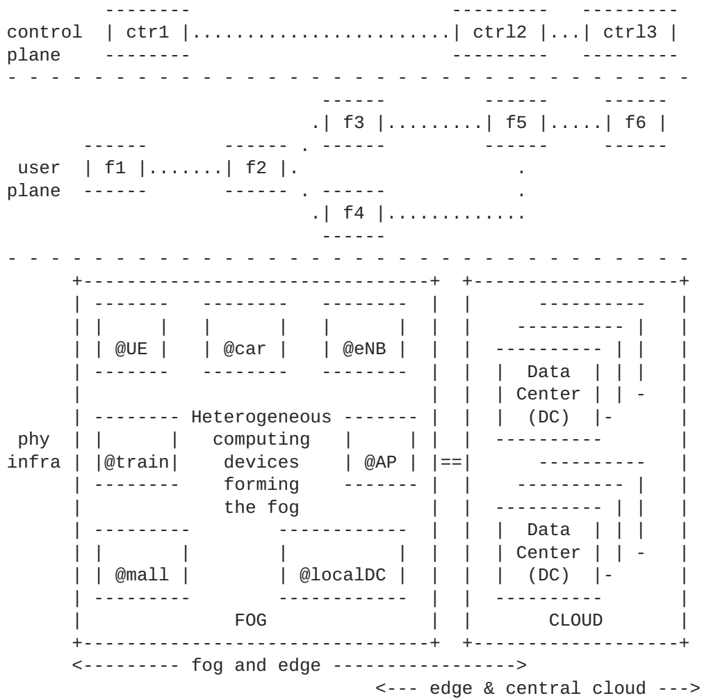
Figure 3: Fog virtualization
