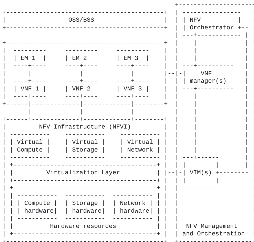
Figure 2: ETSI NFV reference architecture
