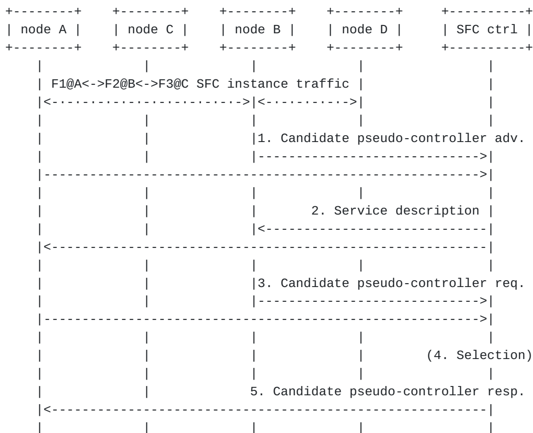
Figure 2: SFC pseudo controller initialization
