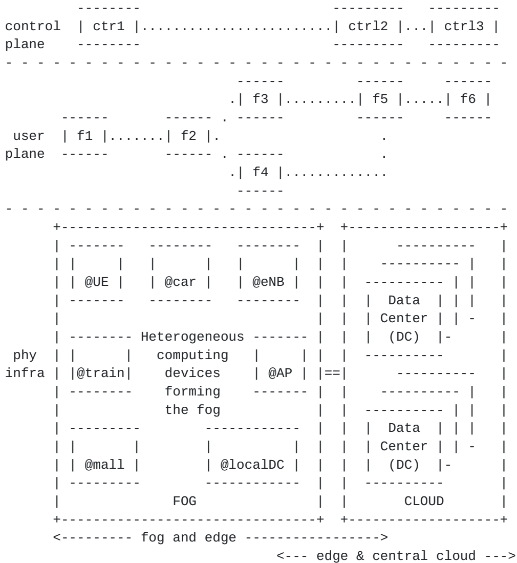
Figure 1: Fog RAN
