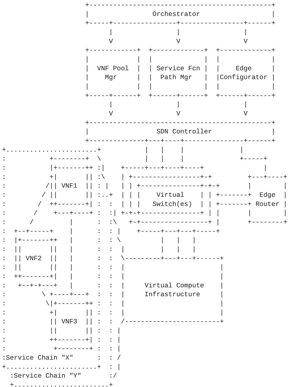
Figure 1: VNF Pool Orchestration Framework Architecture.
