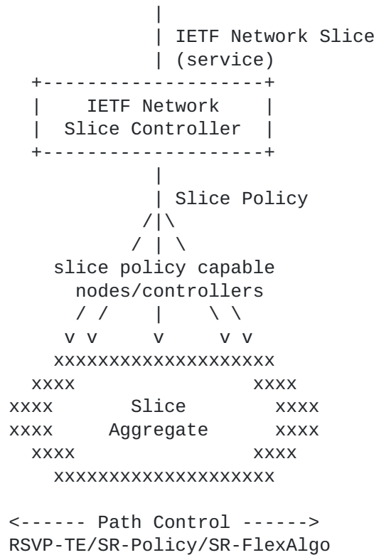
Figure 2: Slice Policy Instantiation.
