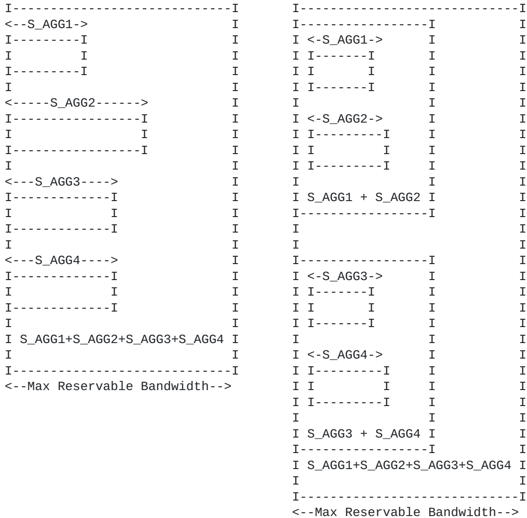
(a) No bandwidth sharing between slice aggregates.
