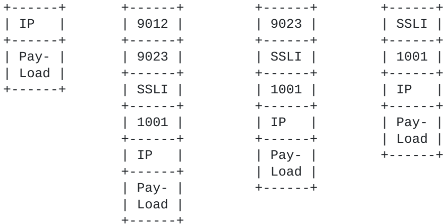
Figure 5: SSLI and bottom SSL at bottom of label stack.
