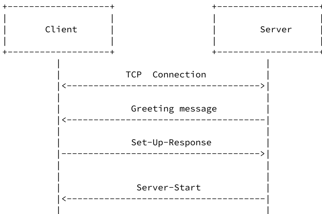
Figure 1. The procedure of O/TWAMP-Control
