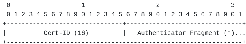
Figure 8: CERTIFICATE frame payload
