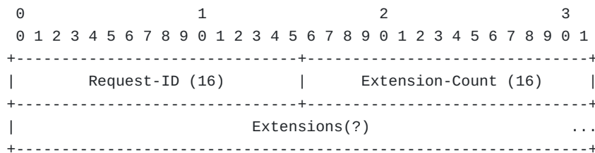
Figure 7: CERTIFICATE_REQUEST frame payload
