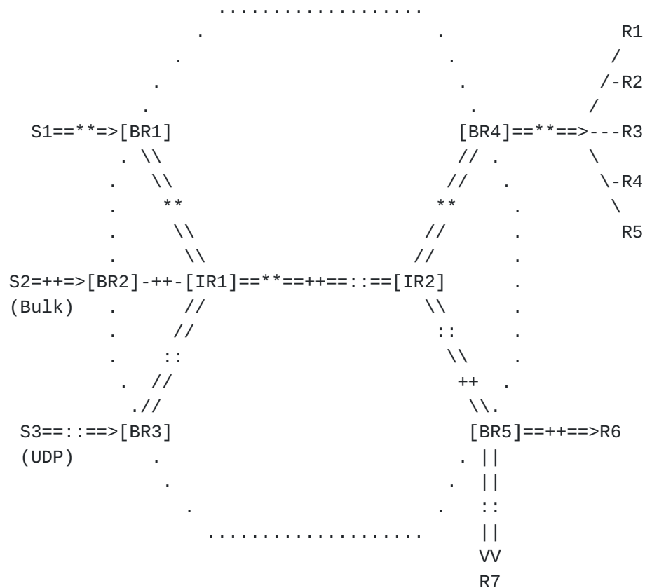
Figure 1: A DiffServ domain with different flows
