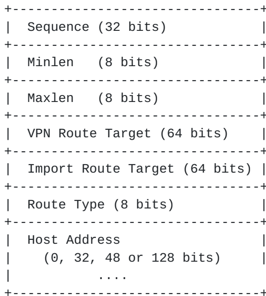
Figure 1: CP-ORF Type-specific Encoding
