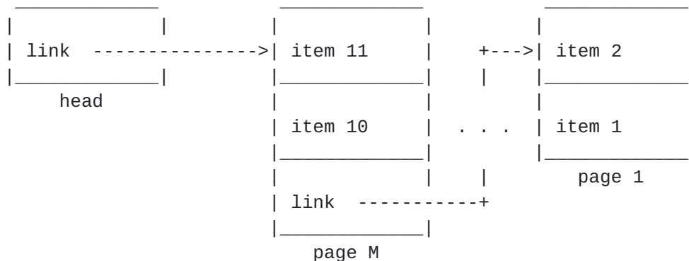
Figure 4: Pagination with stable names
