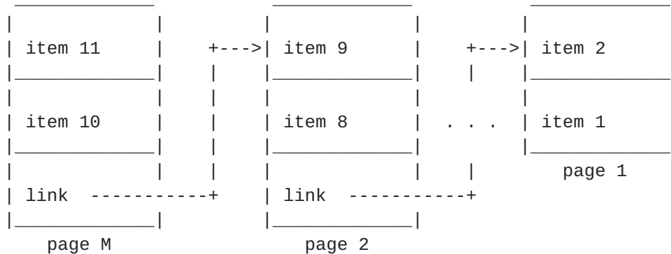
Figure 3: Pagination with stable names
