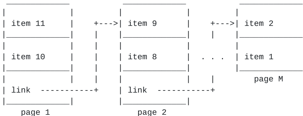
Figure 2: A paginated collection of items
