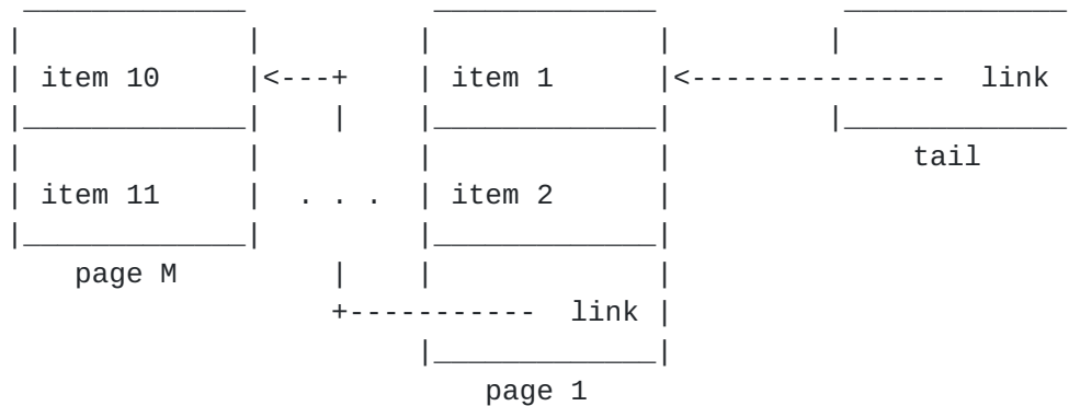
Figure 5: Cursor pattern pictured as pagination
