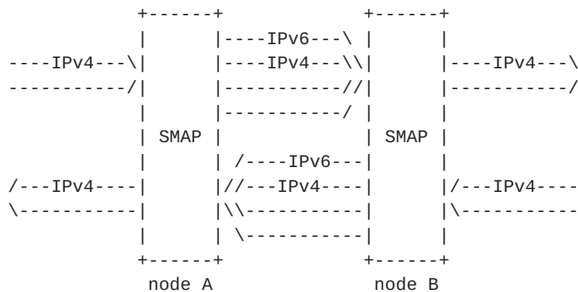
Figure 6: Second Configuration
