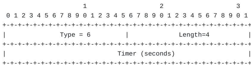
Figure 7: MSF-REBOOT-TIMER sub-TLV
