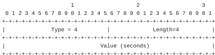
Figure 5: MSF-EPOCH sub-TLV
