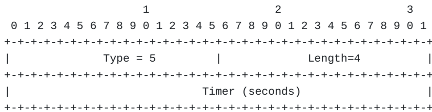
Figure 6: MSF-UNAVAILABILITY-TIMER sub-TLV
