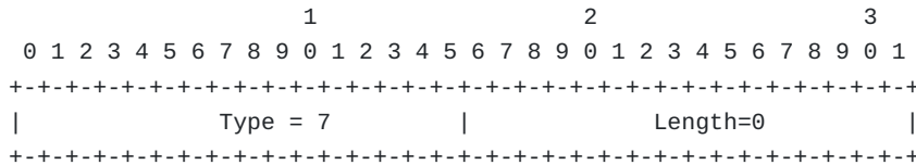
Figure 8: MSF-DIAGNOSIS sub-TLV
