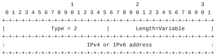
Figure 3: MSF-LOCATOR sub-TLV
