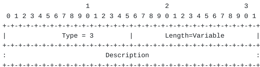
Figure 4: MSF-DESCRIPTION sub-TLV
