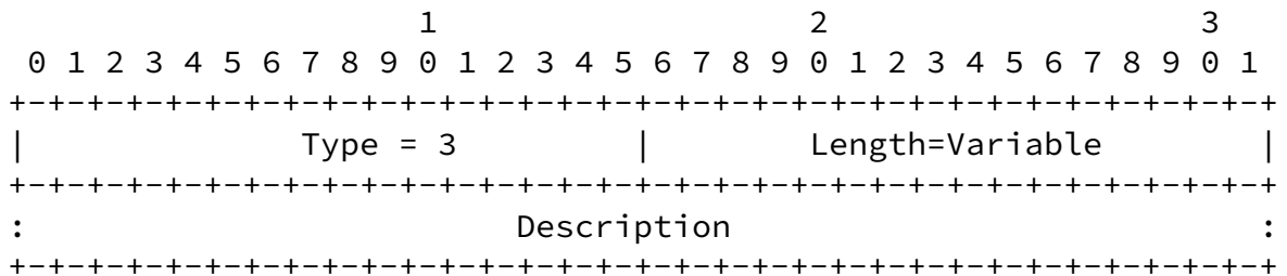
Figure 4: MSF-DESCRIPTION sub-TLV
