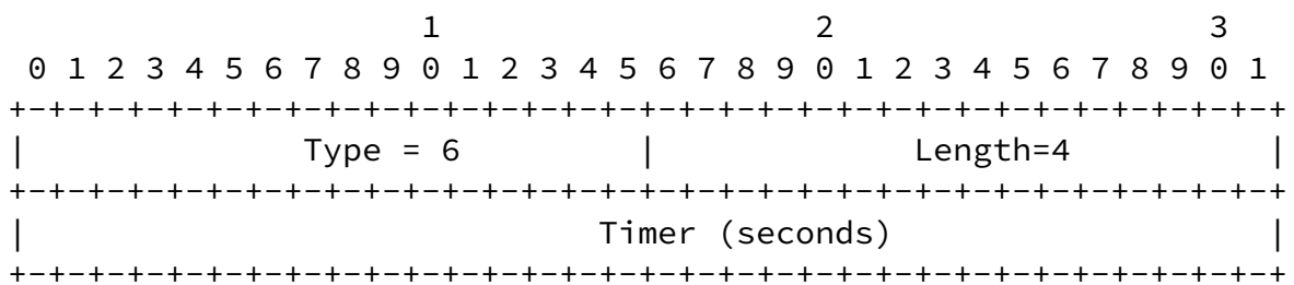
Figure 7: MSF-REBOOT-TIMER sub-TLV
