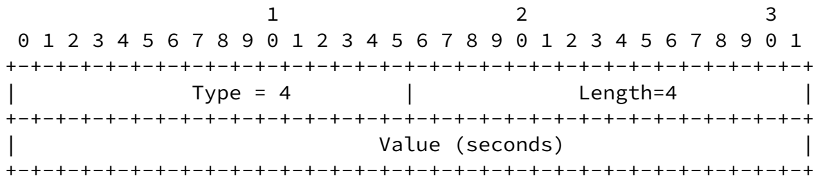
Figure 5: MSF-EPOCH sub-TLV
