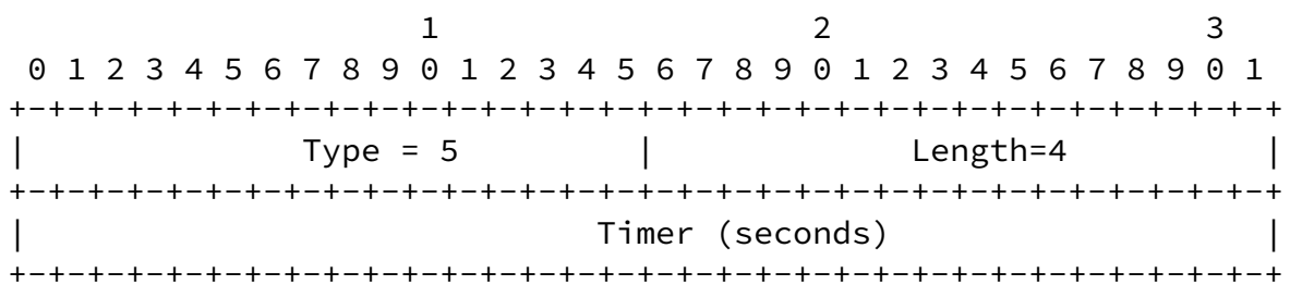
Figure 6: MSF-UNAVAILABILITY-TIMER sub-TLV
