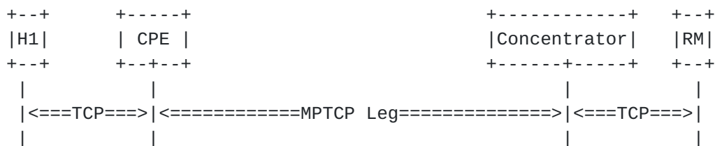
Figure 2: Connection Legs
