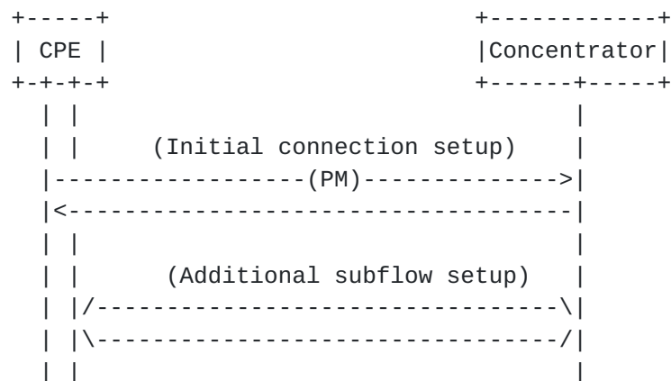
Figure 4: Carrying the Plain Mode Option (Focus on the MPTCP Leg)
