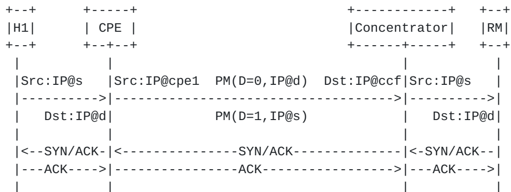
Figure 8: Example of Outgoing SYN with Source Address Preservation
