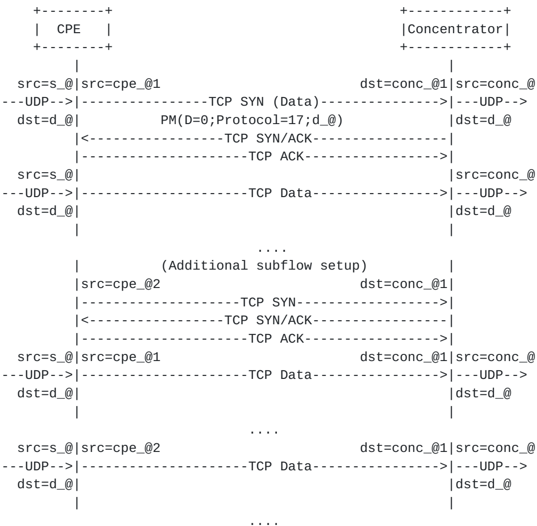
Figure 6: Distributing UDP packets over multiple paths (2)
