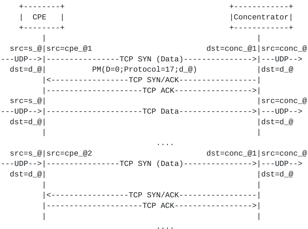
Figure 5: Distributing UDP packets over multiple paths (1)
