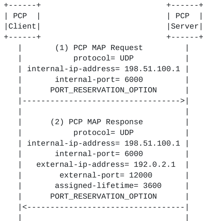
Figure 4: Flow Example of a PCP Server supporting the option but not honoring the hinted external port
