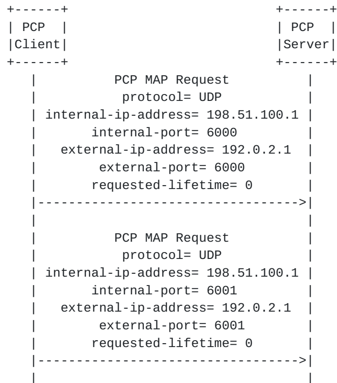
Figure 5: Flow example to delete the mappings
