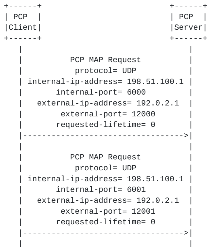
Figure 6: Flow example to delete the mappings (2)
