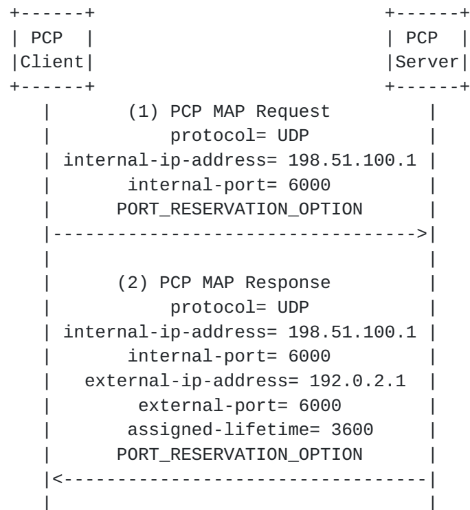
Figure 3: Flow Example of a PCP Server supporting the option and honoring the hinted external port
