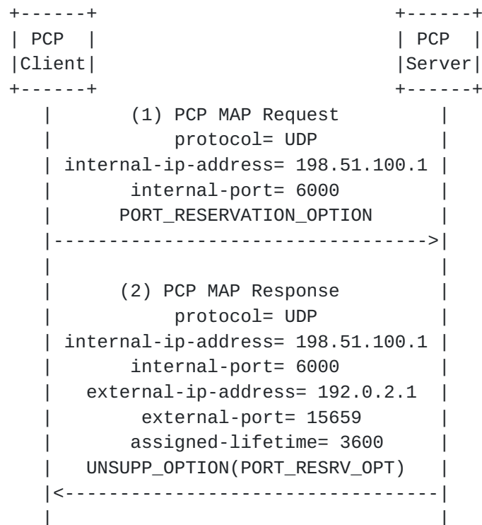
Figure 2: Flow Example of a PCP Server which does not support the Port Reservation Option
