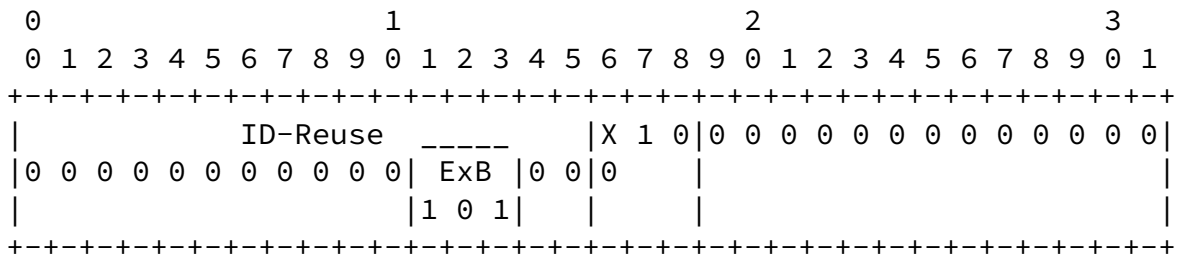
Figure 6: Example of Experimental Reuse of Octets 5 & 6 Without Requiring RC=1
