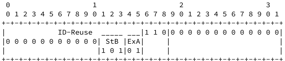
Figure 5: Example of Reuse of Octets 5 & 6 using RC=1
