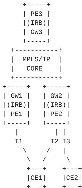
Figure 2. EVPN-IRB Port-active load-balancing
