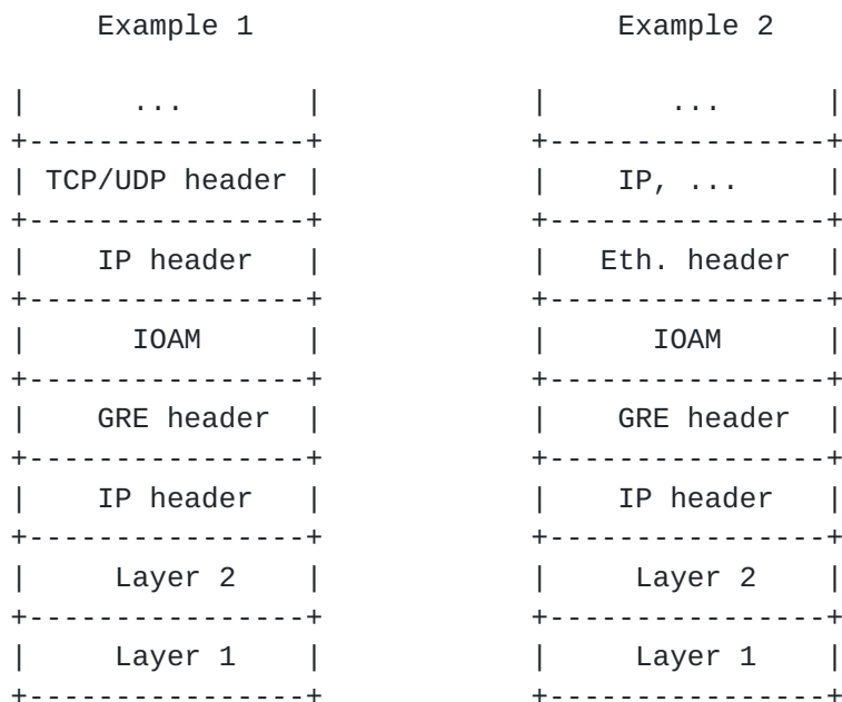
Figure 2: GRE with IOAM example
