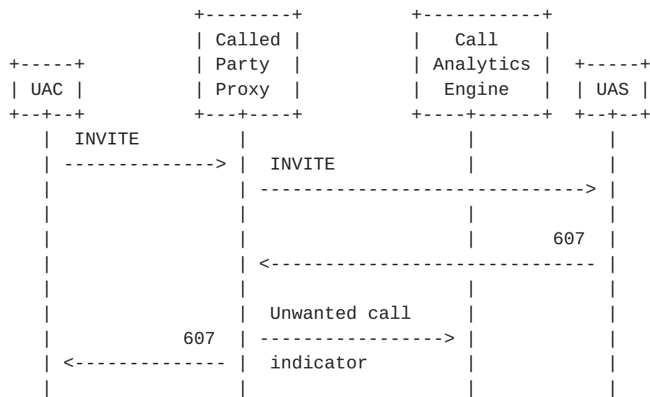
Figure 2: Unwanted (607) Ladder Diagram
