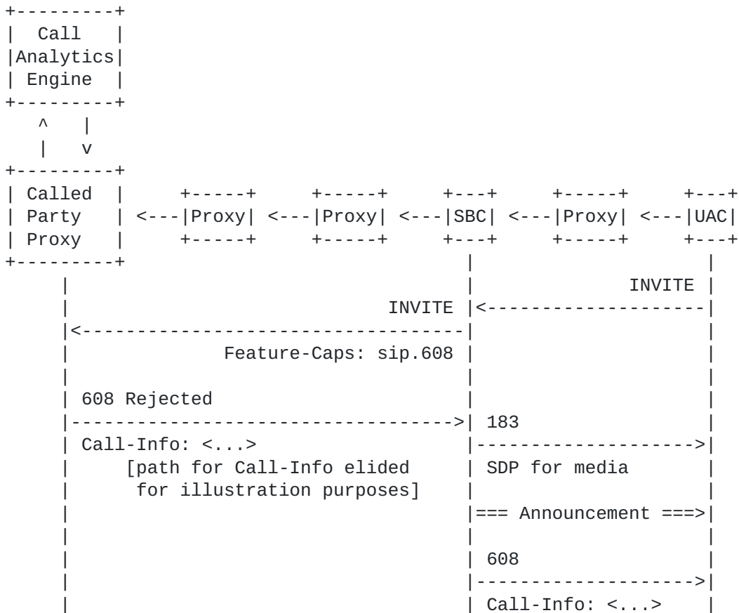
Figure 5: Legacy Operation
