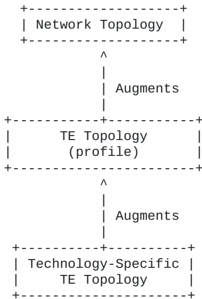
Figure 6: Augmenting the TE Topology Model
