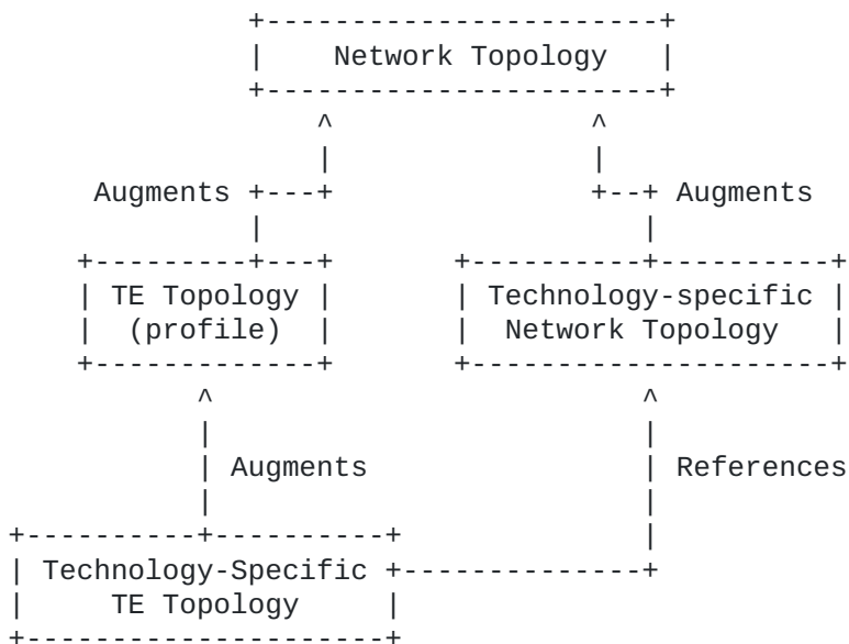
Figure 8: Augmenting both the Network and TE Topology Models
