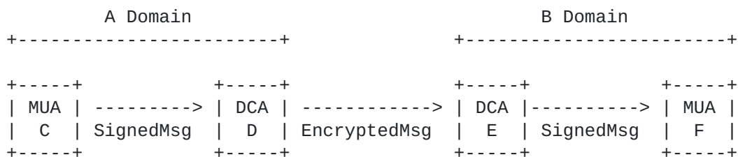
Figure 1: Architecture of Secure Headers
