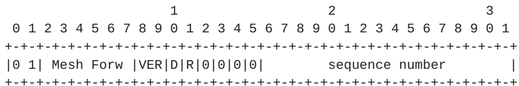
Figure 3: Header for DFF data Packets
