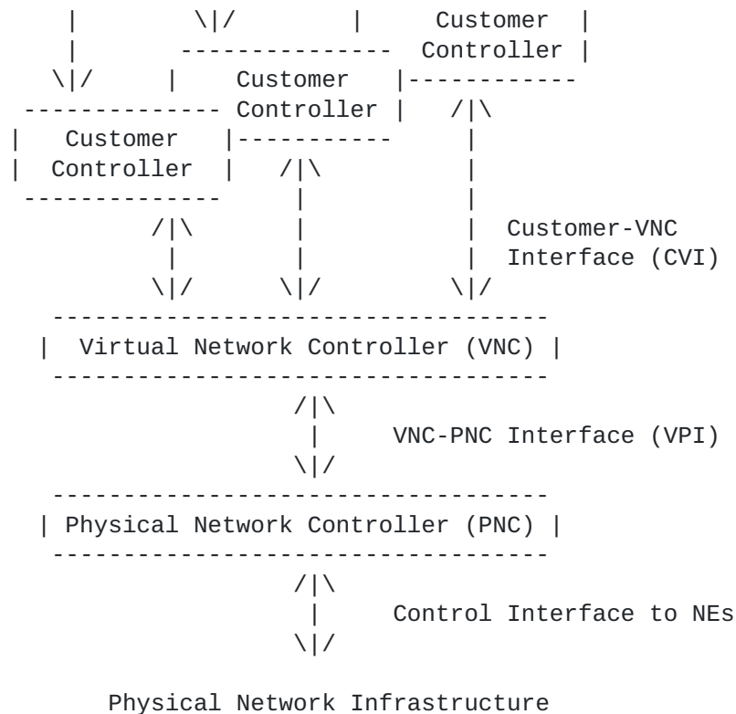
Figure 2: Control and Interface Architecture for ACTN.
