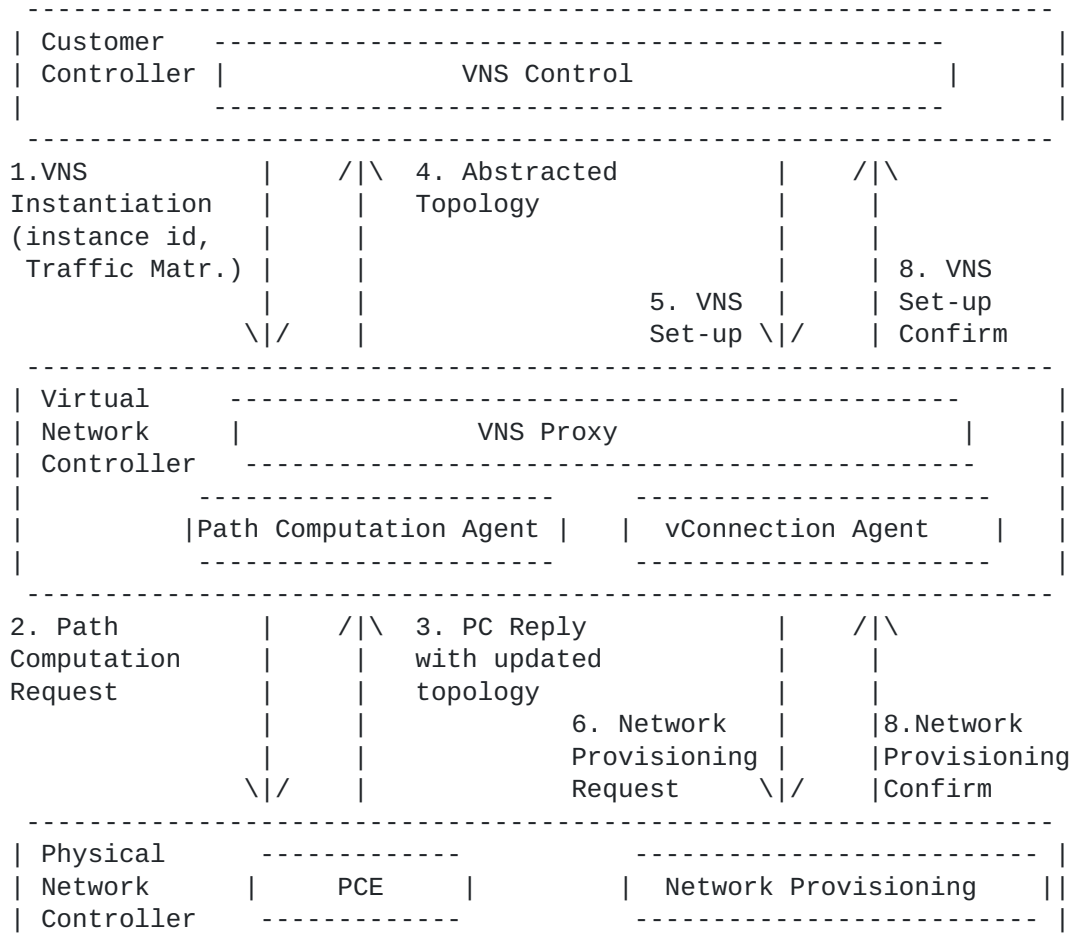
Figure 5. Workflows across Customer Controller, VNC and PNC
