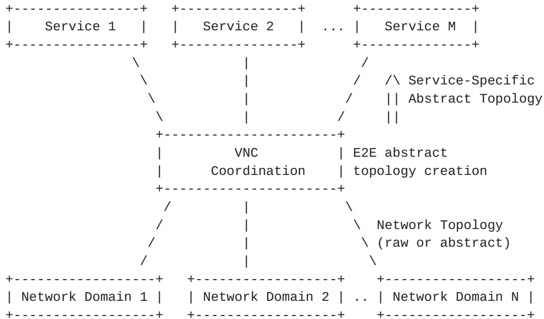
Figure 3: Multi-domain three-tier relationship
