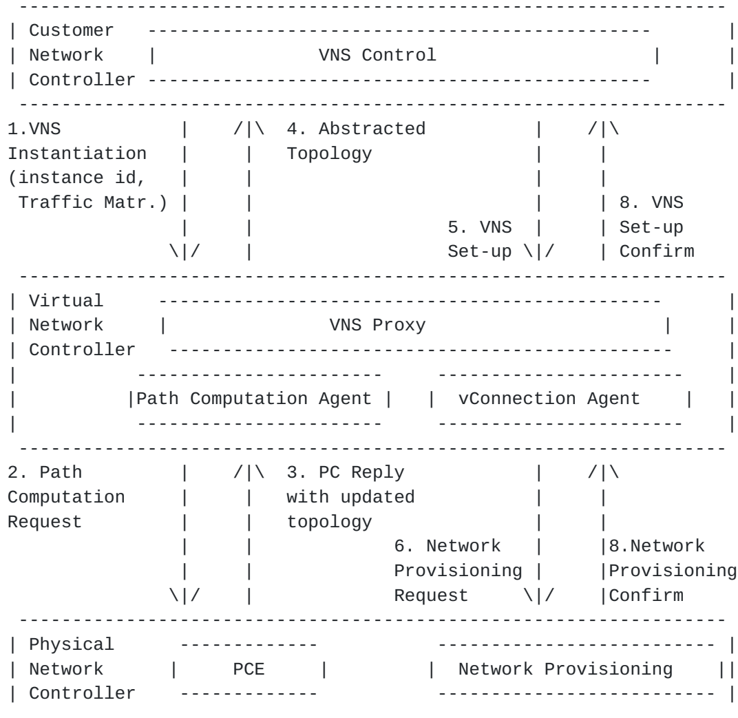
Figure 8. Workflows across CNC, VNC and PNC
