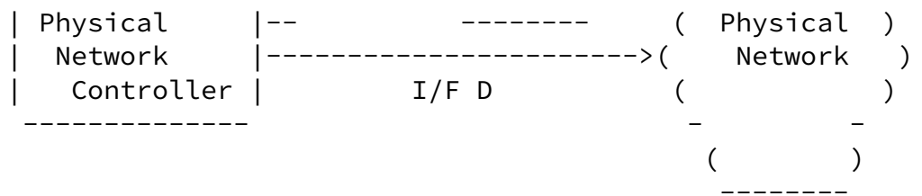
Figure 5. ACTN Interfaces
