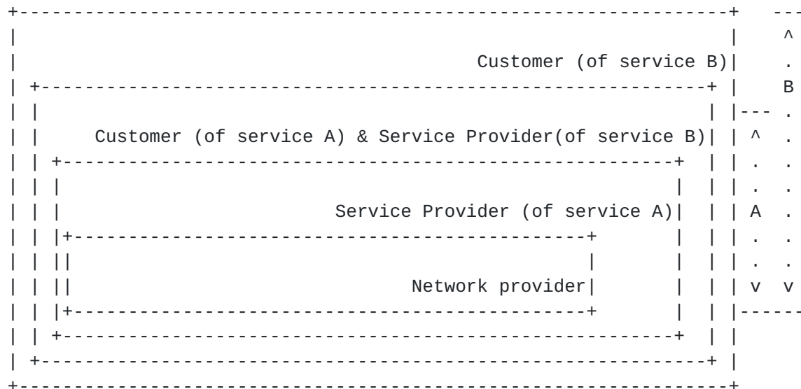
Figure 1: Network Recursiveness.
