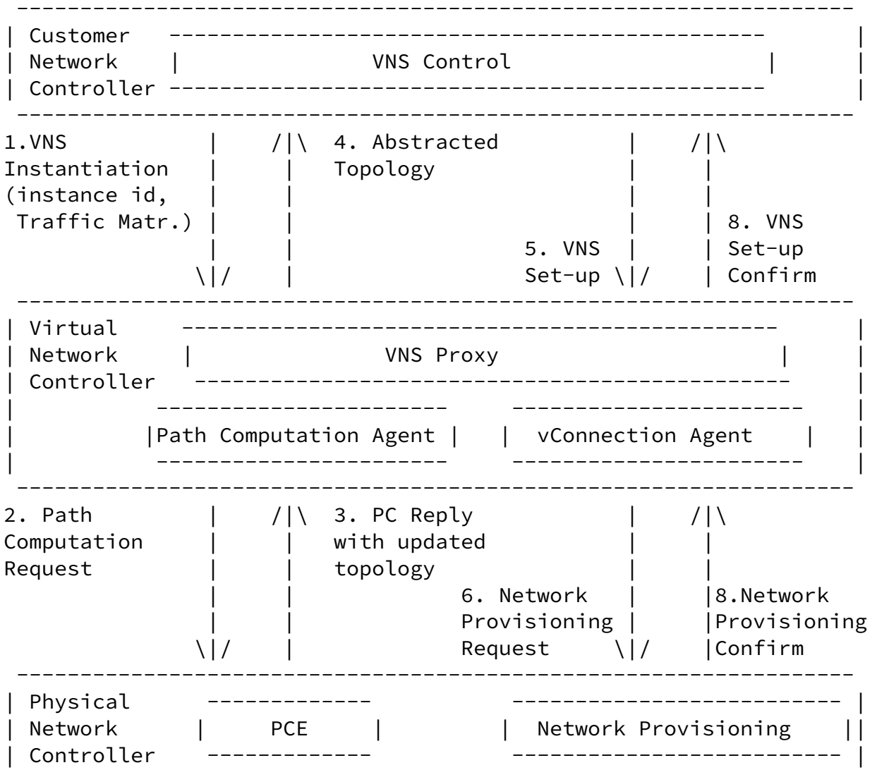
Figure 8. Workflows across CNC, VNC and PNC
