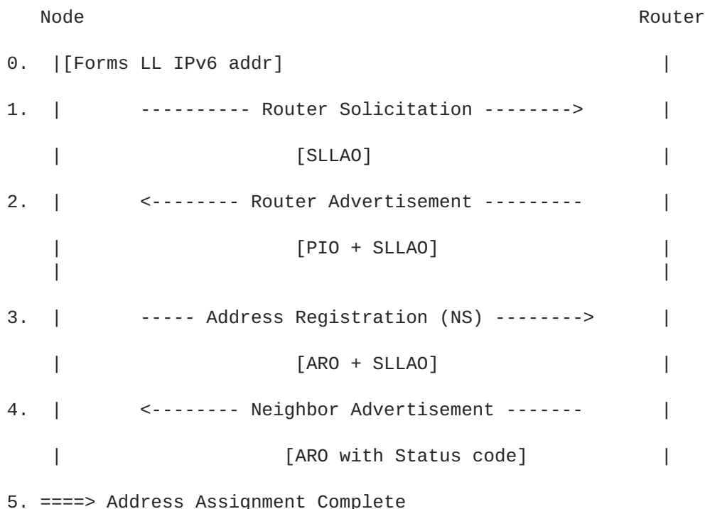
Figure 1: Neighbor Discovery Address Registration and bootstrapping
